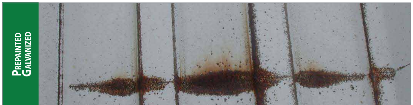
Comparison of drip edge corrosion on a 20 year old building in severe acid rain environment, Pennsylvania.
